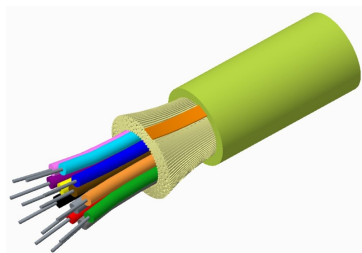
LazrSPEED® Low Smoke Zero Halogen Riser Distribution Cable, 12 fiber single-unit, OM4
